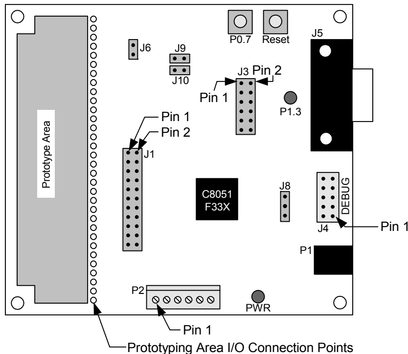
Figure 3. C8051F330 Target Board
