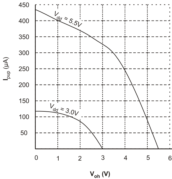
Weak Pull-up Source Current I_{pup} (Ports A/B/C/D/E)
