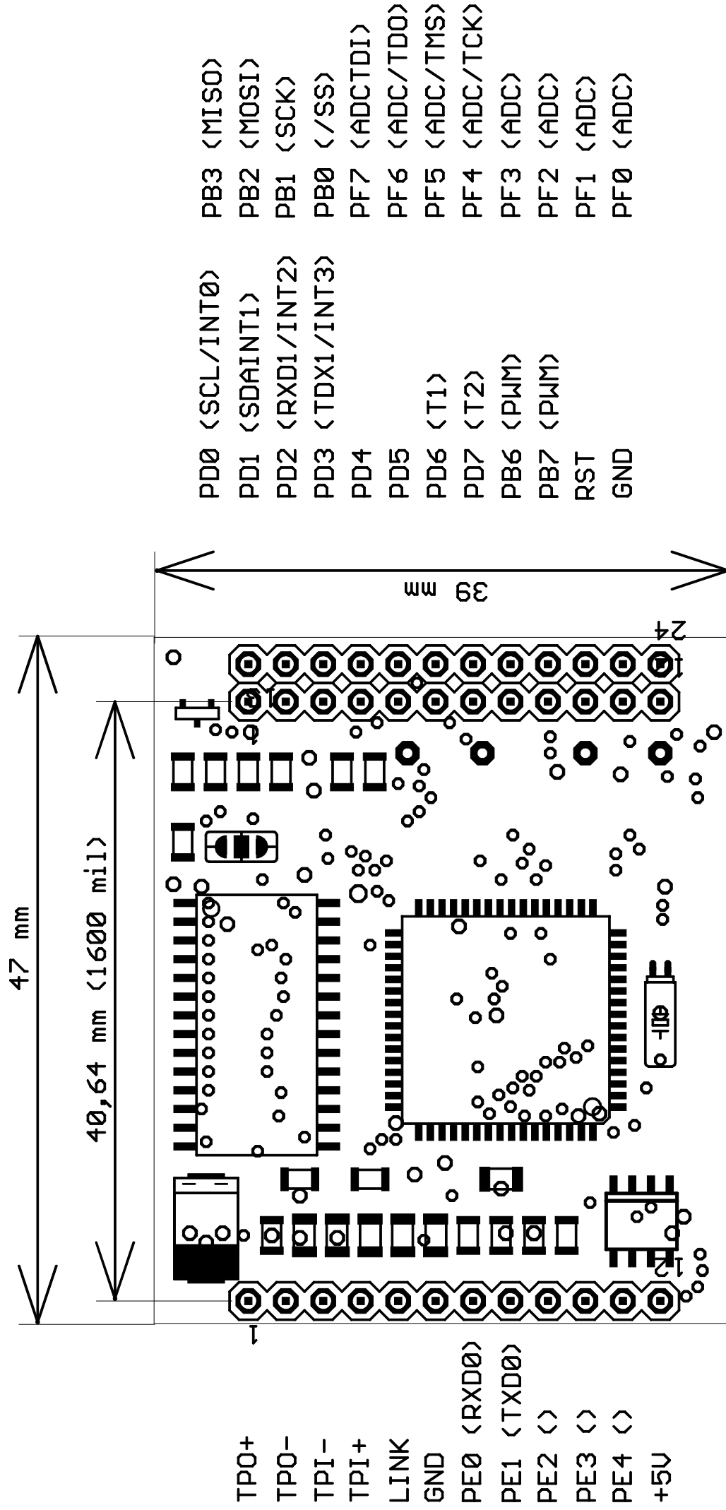
Charon II embedded Ethernet module (Ethernet compatible)
