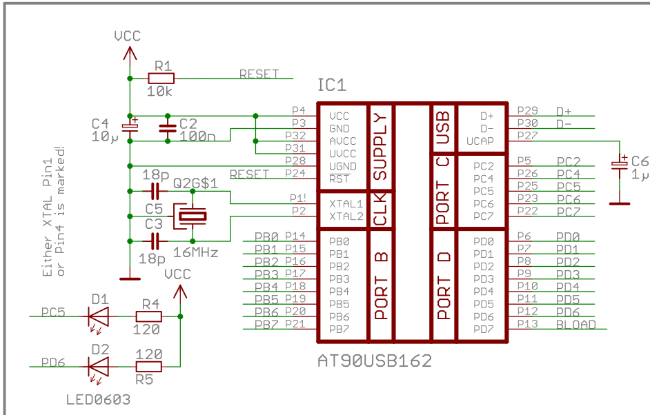
MCU_CIRCUIT
