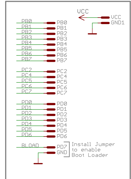
PROTOTYPING_AREA
