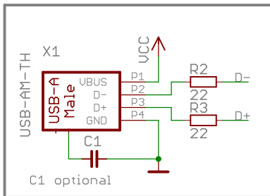
USB_CONNECTOR
